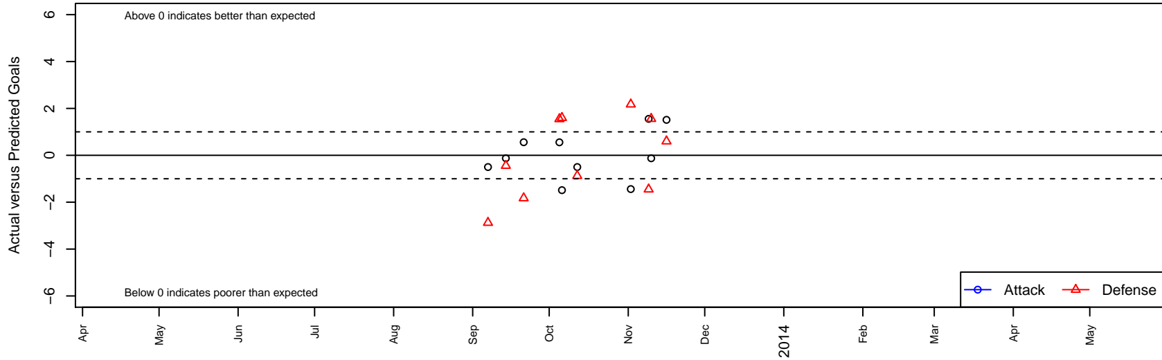
Merced United FC B00 Dots are actual minus expected GF (blue circles) and GA (red triangles). Blue line is smoothed change in attack strength. Red is smoothed change in defense strength.
